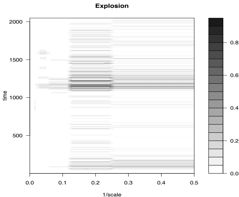
Fig. 4.25. Time-scale image (scalogram) of the explosion series.
