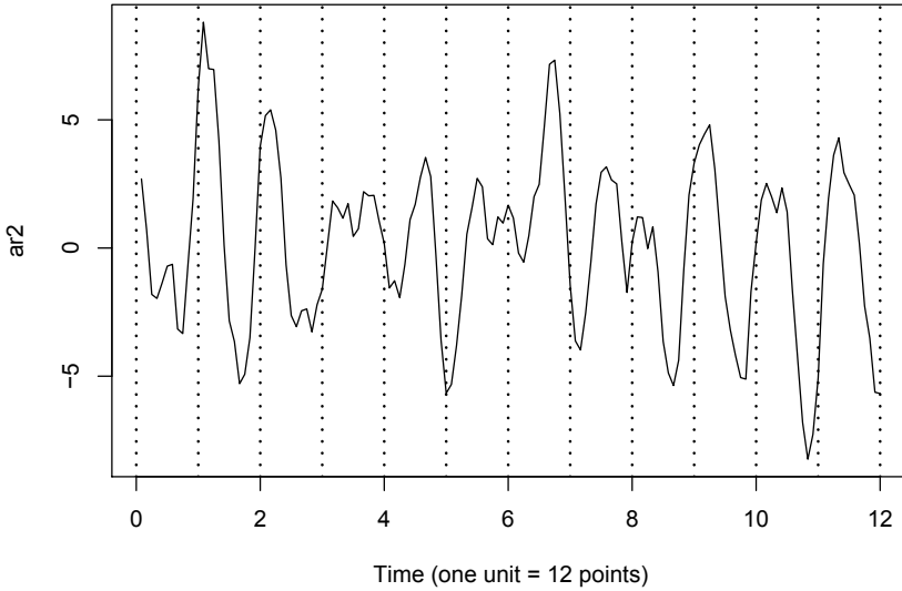
Fig. 3.3. Simulated AR(2) model, n = 144 with \phi_1 = 1.5 and \phi_2 = -.75 .
