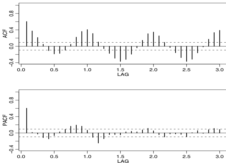
Fig. 5.10. Sample ACF and PACF of SOI.
