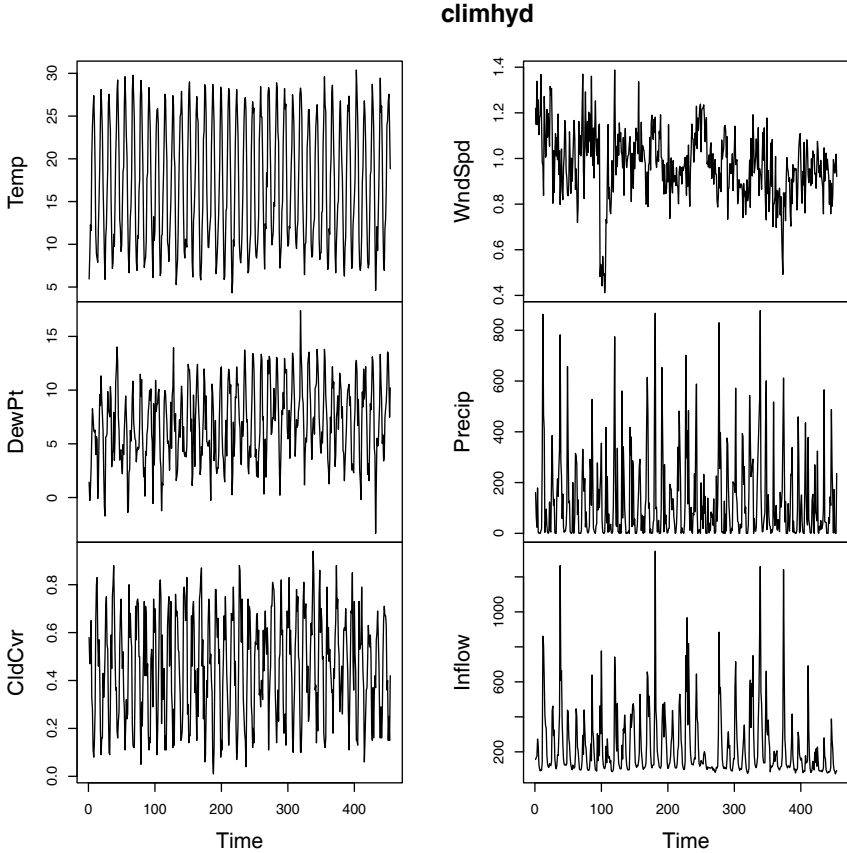
Fig. 7.3. Monthly values of weather and inflow at Lake Shasta.
