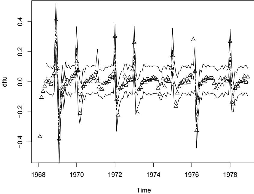
Fig. 5.8. First differenced U.S. monthly pneumonia and influenza deaths (triangles); one-month-ahead predictions (dashed line) with \pm 2 prediction error bounds (solid line).
