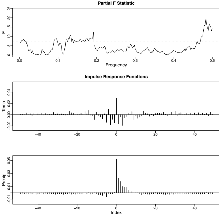
Fig. 7.5. Partial F -statistics [top] for testing whether temperature adds to the ability to predict Lake Shasta inflow when precipitation is included in the model. The dashed line indicates the .001 FDR level and the solid line represents the corresponding quantile of the null F distribution. Multiple impulse response functions for the regression relations of temperature [middle] and precipitation [bottom].
