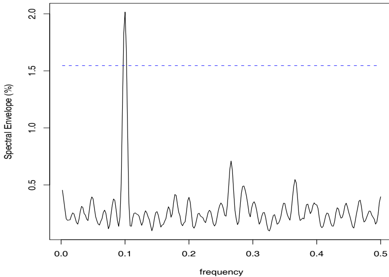
Fig. 7.29. Spectral envelope with respect to \mathcal{G} = \{x, \sqrt{x}, \sqrt[3]{x}\} of data generated from (7.188).
