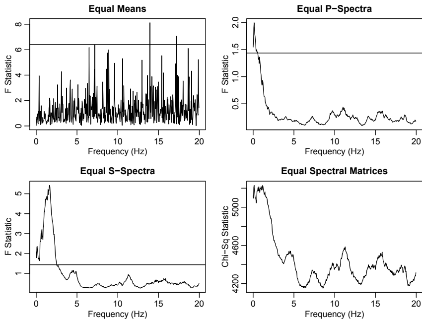
Fig. 7.12. Tests for equality of means, spectra, and spectral matrices for the earthquake and explosion data p = 2, L = 21, n = 1024 points at 40 points per second.
