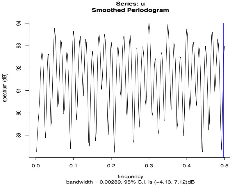
Fig. 7.28. Periodogram, in decibels, of the data generated from (7.188) after tapering by a cosine bell.
