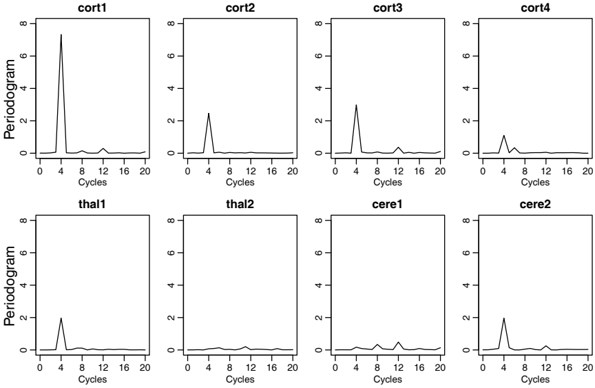
Fig. 7.17. The individual periodograms of x_{tk} , for k = 1, \dots, 8 , in Example 7.14.
