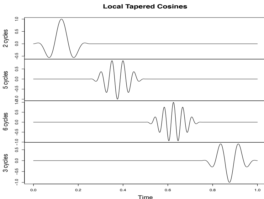
Fig. 4.19. Local, tapered cosines at various frequencies.
