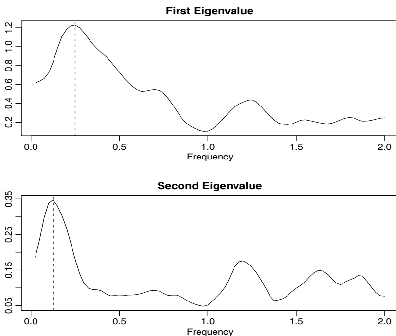
Fig. 7.22. The first, \hat{\lambda}_1(\omega) , and second, \hat{\lambda}_2(\omega) , eigenvalues of the estimated spectral matrix \hat{f}_{xx}(\omega) . The vertical dashed lines are shown at \omega = .25 and .125 , respectively.
