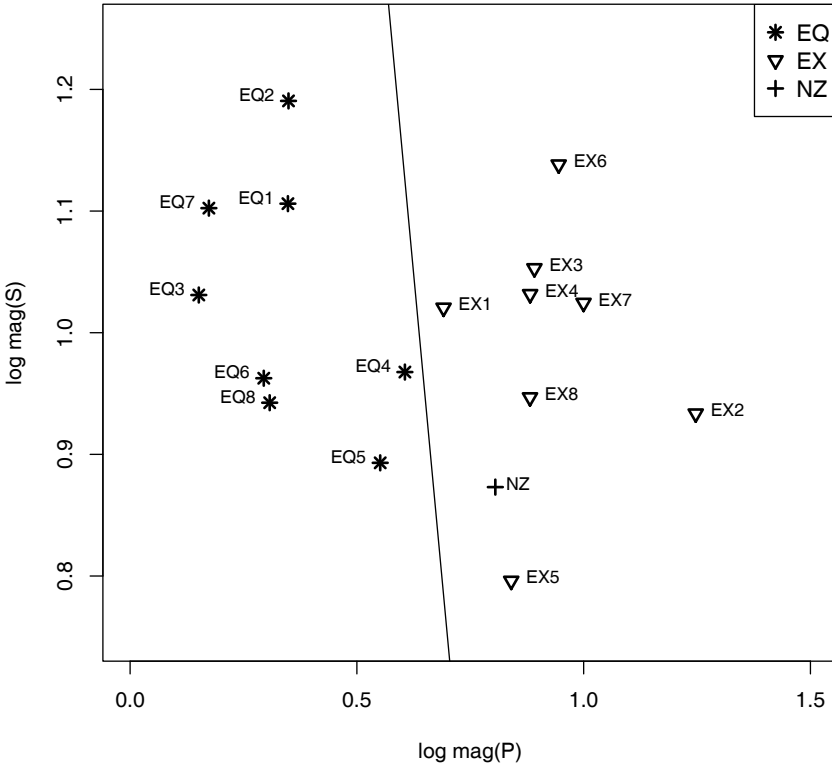
Fig. 7.13. Classification of earthquakes and explosions based on linear discriminant analysis using the magnitude features.
