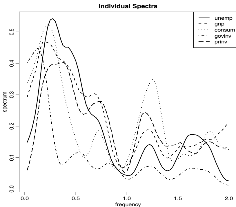
Fig. 7.20. The individual estimated spectra (scaled by 1000) of each series show in Figure 7.19 in terms of the number of cycles in 160 quarters.
