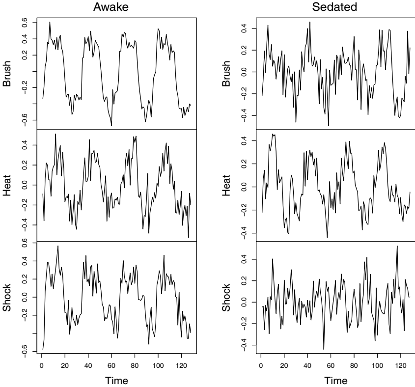
Fig. 7.1. Mean response of subjects to various combinations of periodic stimuli measured at the cortex (primary somatosensory, contralateral). In the first column, the subjects are awake, in the second column the subjects are under mild anesthesia. In the first row, the stimulus is a brush on the hand, the second row involves the application of heat, and the third row involves a low level shock.
