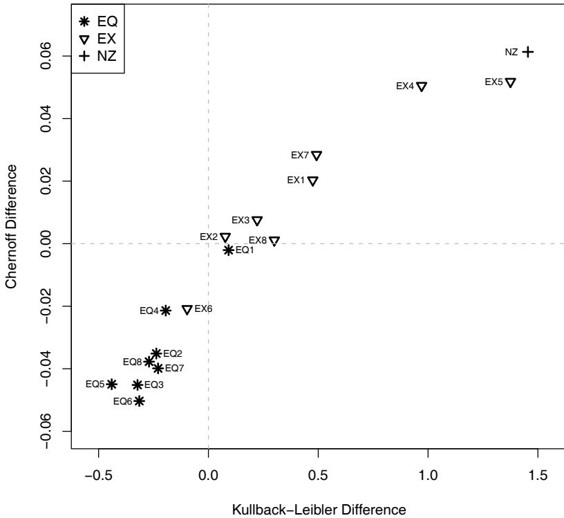
Fig. 7.15. Classification (by quadrant) of earthquakes and explosions using the Chernoff and Kullback-Leibler differences.
