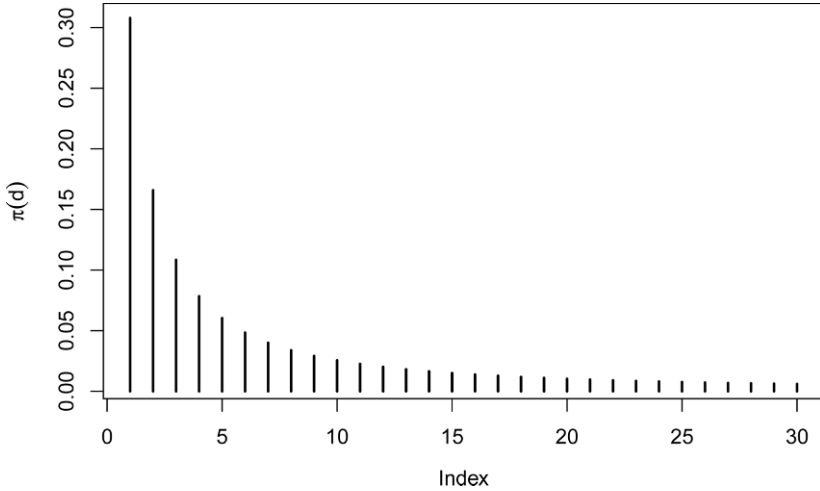
Fig. 5.2. Coefficients \pi_j(.384), j = 1, 2, \dots, 30 in the representation (5.7).
