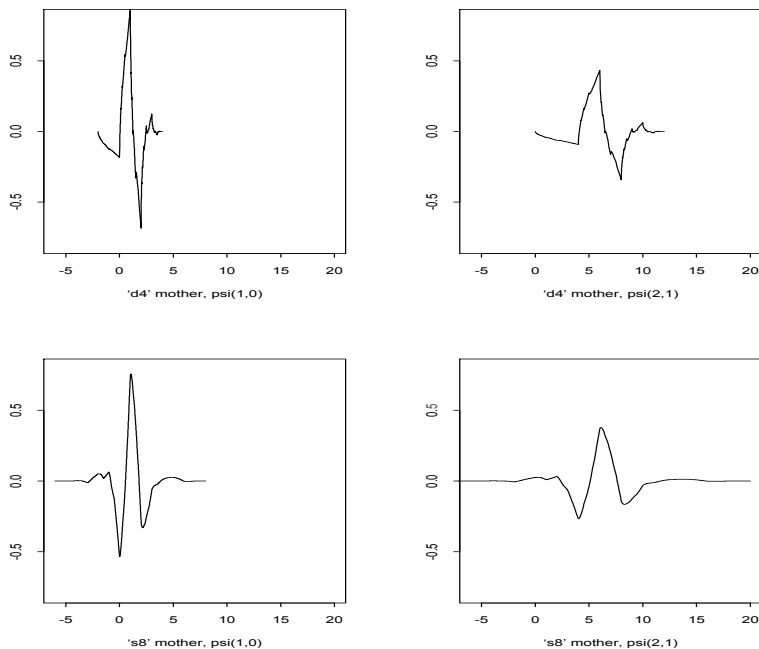
Fig. 4.21. Scaled and translated daubelet4 wavelets, \psi_{1,0}(t) and \psi_{2,1}(t) (top row); scaled and translated symmlet8 wavelets, \psi_{1,0}(t) and \psi_{2,1}(t) (bottom row).
