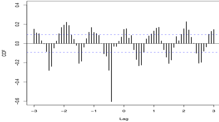
Fig. 5.11. Sample CCF of the prewhitened, detrended SOI and the similarly transformed Recruitment series; negative lags indicate that SOI leads Recruitment.
