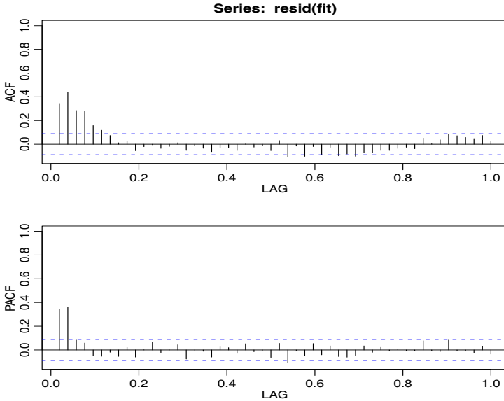
Fig. 5.9. Sample ACF and PACF of the mortality residuals indicating an AR(2) process.
