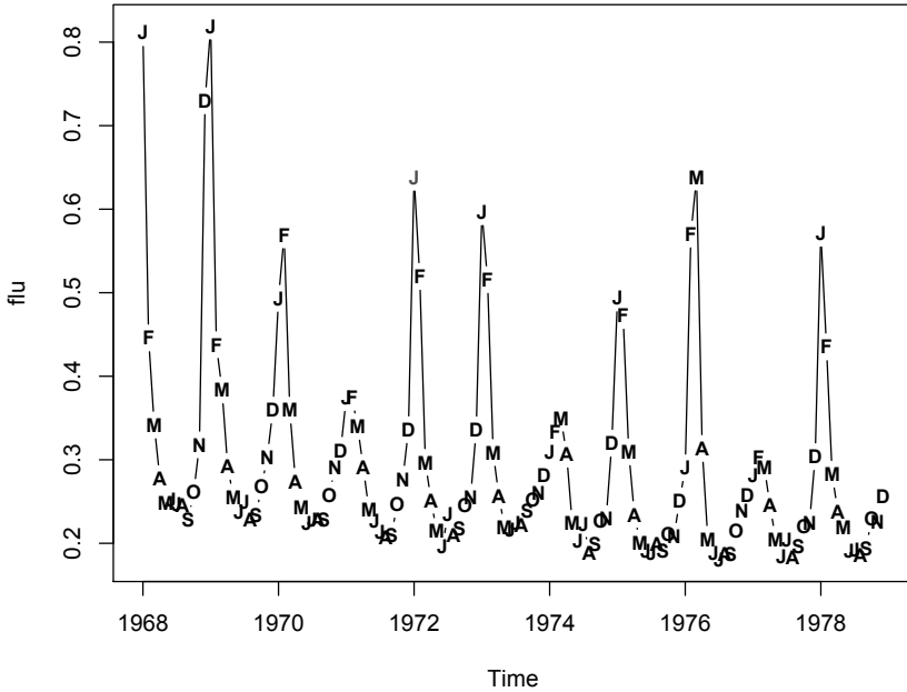
Fig. 5.7. U.S. monthly pneumonia and influenza deaths per 10,000.
