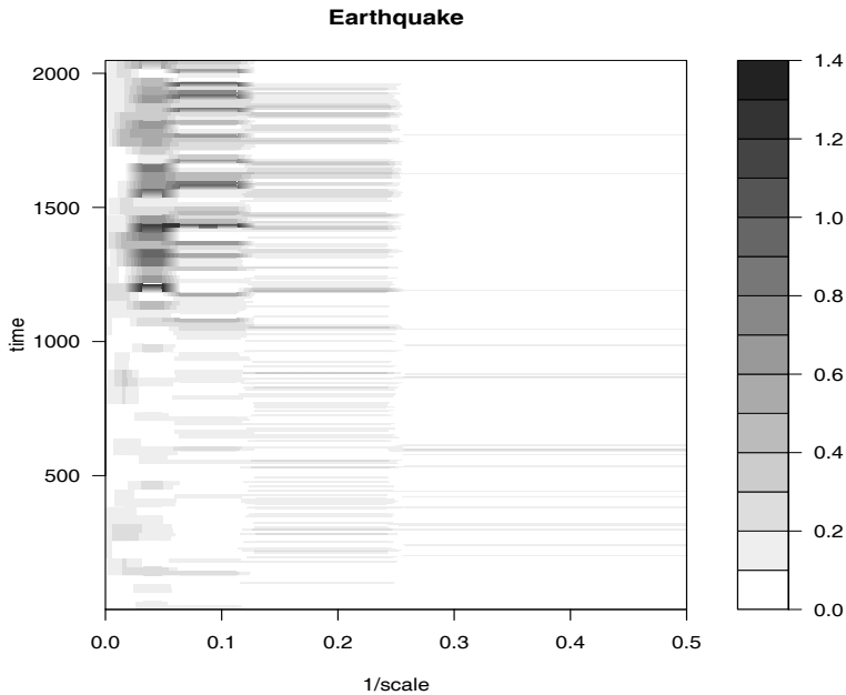
Fig. 4.24. Time-scale image (scalogram) of the earthquake series.
