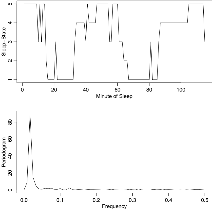
Fig. 7.23. [Top] Time plot of the EEG sleep state data in Table 7.10 using the scaling in (7.179). [Bottom] Periodogram of the EEG sleep state data in Figure 7.23 based on the scaling in (7.179). The peak corresponds to a frequency of approximately one cycle every 60 minutes.
