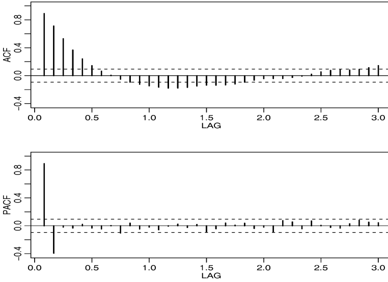
Fig. 5.12. ACF and PACF of the estimated noise \hat{\eta}_t departures from the transfer function model.
