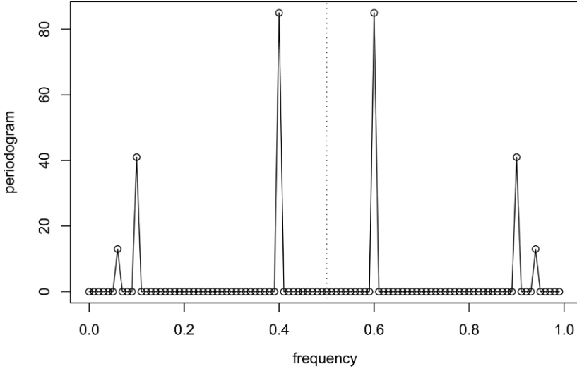
Fig. 4.2. Periodogram of the data generated in Example 4.1.
