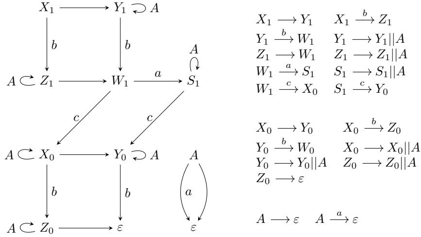
Figure 2.1: Combining two copies of the context-free grammar from Example 11 yields X_1 \stackrel{L}{\approx}_{\omega+\omega} Y_1 \not\approx X_1 .
